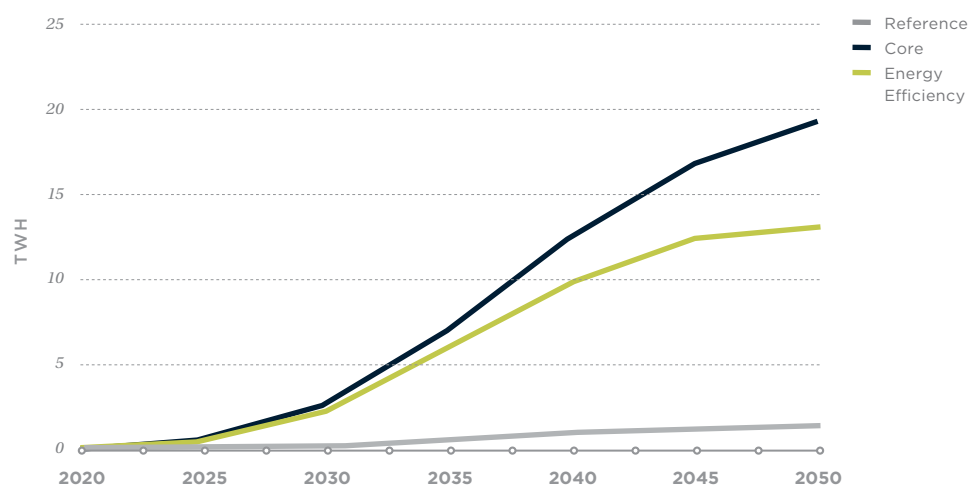
FIGURE 18. ELECTRICITY LOAD FROM TRANSPORTATION ELECTRIFICATION IN REFERENCE, CORE AND ENERGY EFFICIENCY SCENARIOS
