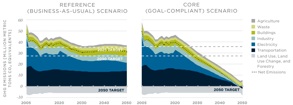
ES FIGURE 1. REFERENCE AND CORE SCENARIO GREENHOUSE GAS EMISSIONS BY SECTOR, WITH COMPARISON TO NEVADA’S 2025, 2030, AND 2050 GOALS
