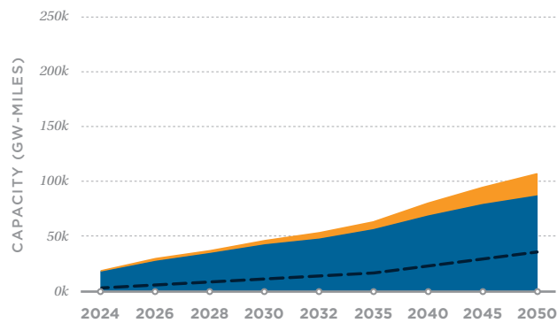
CUMULATIVE INSTALLED CAPACITY: RESTRICTED BUILD-OUT
